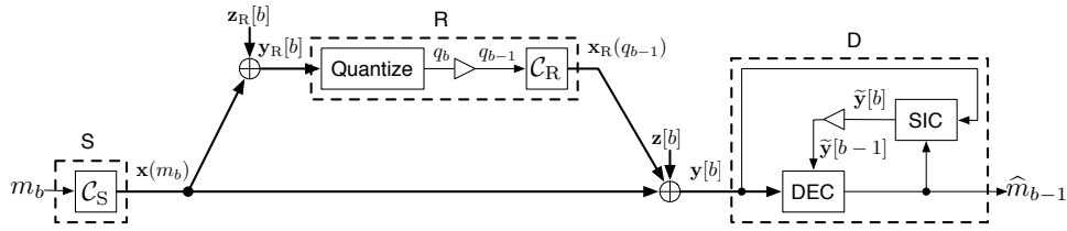
Fig. 4. System architecture for block index b .
