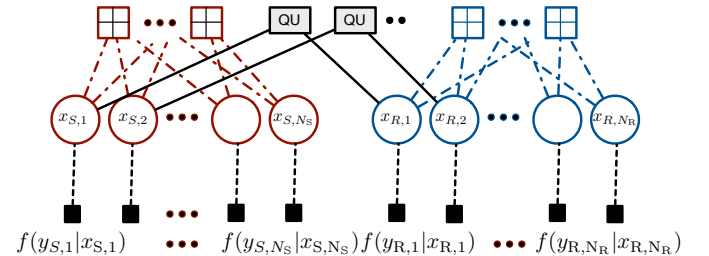
Fig. 6. Simplified factor graph with one-bit scalar quantizer, that is, \alpha_i = \{i\} for i = 1, 2, \dots, fN_S .
