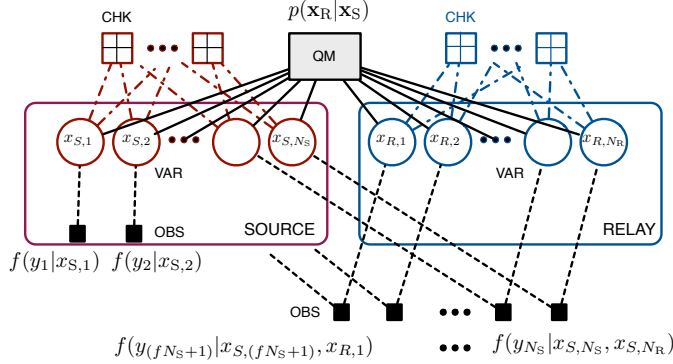
Fig. 2. Factor graph
