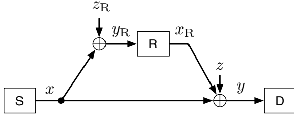
Fig. 1. Half-Duplex Gaussian Relay Channel
