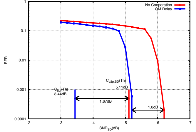
Fig. 9. 16QAM Simulation Results for q_{SR} = 2 , q_{RD} = 1 , N_S = 20400 , N_R = 13600 , f = \frac{1}{3} , r_S = r_R = 0.5
