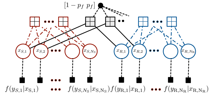
Fig. 7. Equivalent factor graph of that in Fig. 6
