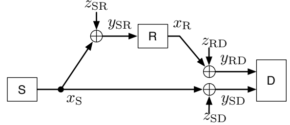
Fig. 5. Equivalent channel model
