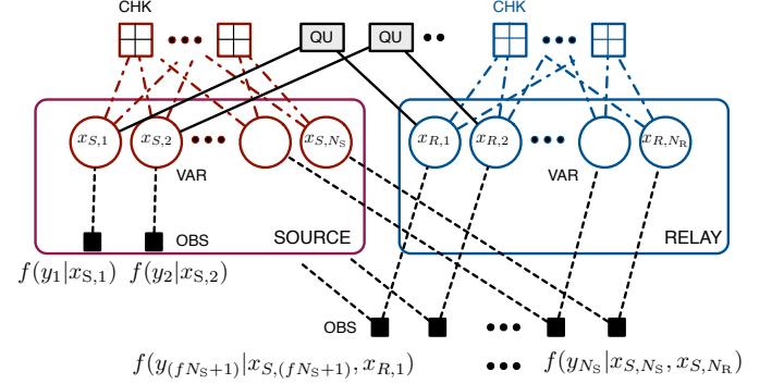
Fig. 3. Factor graph: Systematic code at relay and scalar quantizer.
