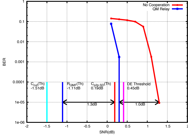
Fig. 8. Simulation results for q_{SR} = 2 , q_{RD} = 1 , N_S = 20400 , N_R = 13600 , f = \frac{1}{3} , r_S = r_R = 0.5
