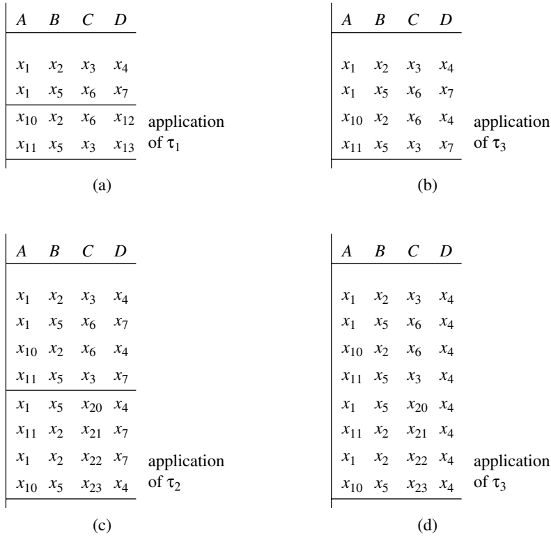
Figure 10.3: Parts of a chasing sequence
