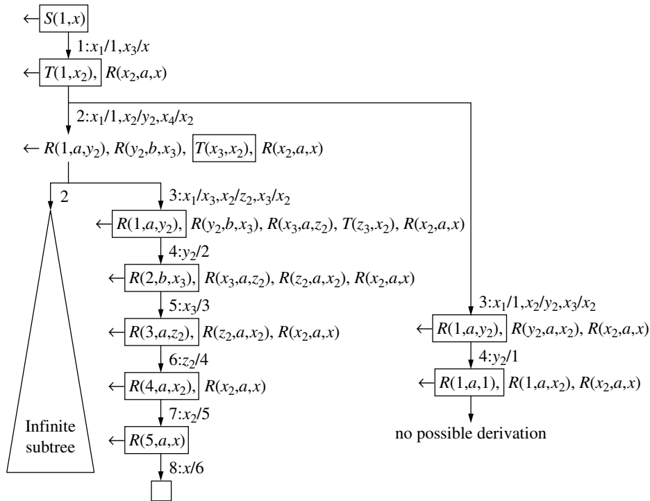
Figure 12.6: SLD tree
