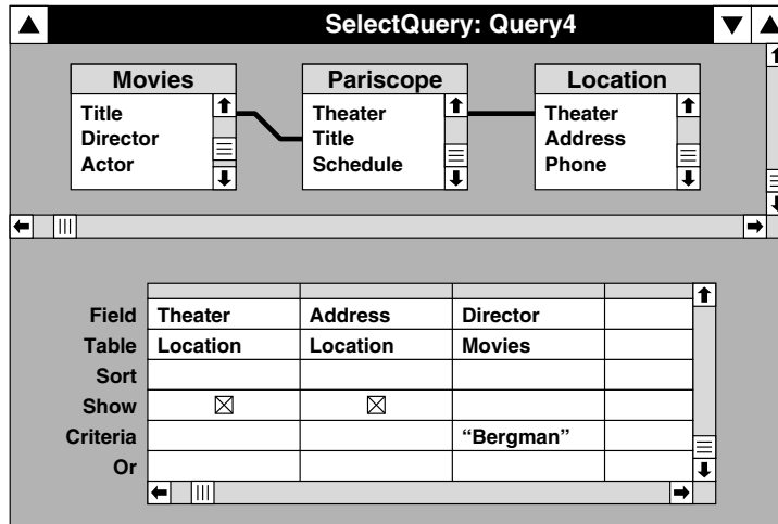
Figure 7.4: Example query in Access
