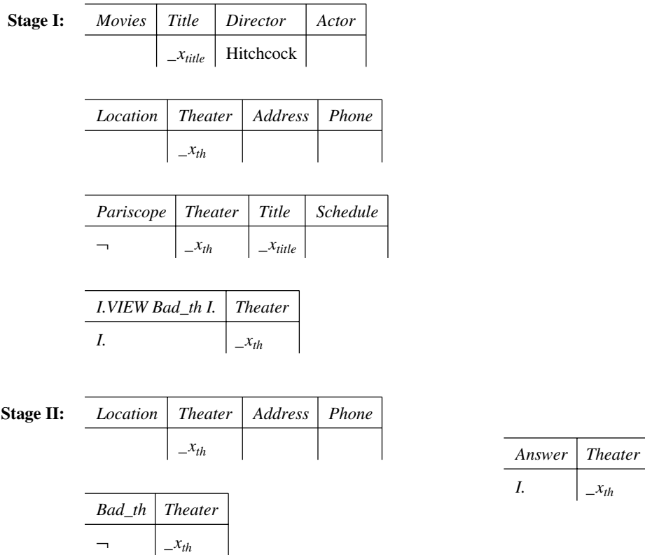
Figure 7.3: Illustration of relational completeness of QBE
