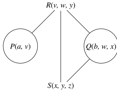
Figure 6.3: A sip graph
