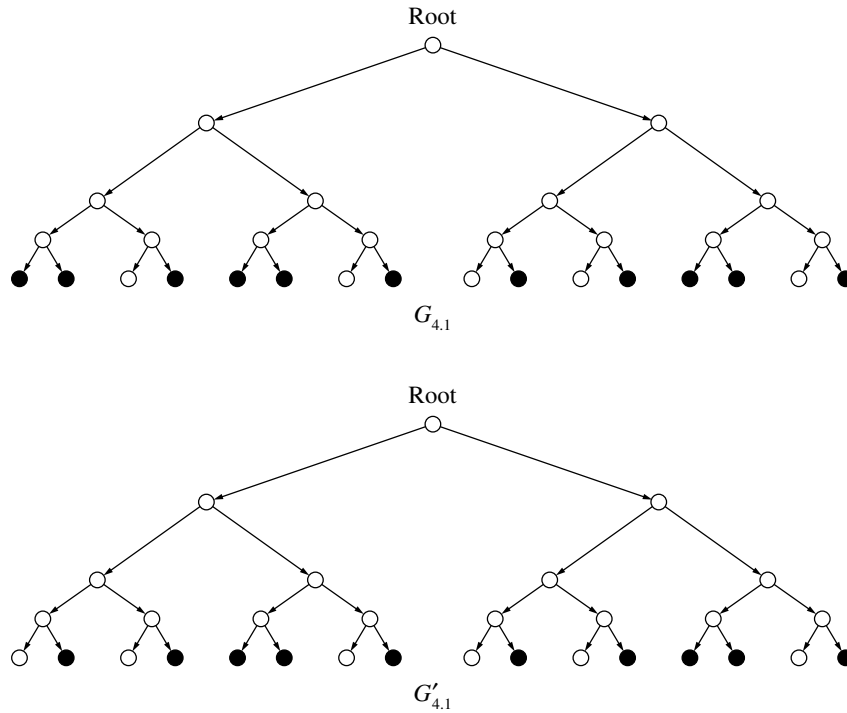
Figure 15.2: Game trees
