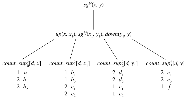
(b) Alternative QSQ "template," using indices
