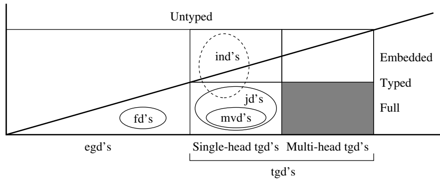
Figure 10.1: Dependencies
