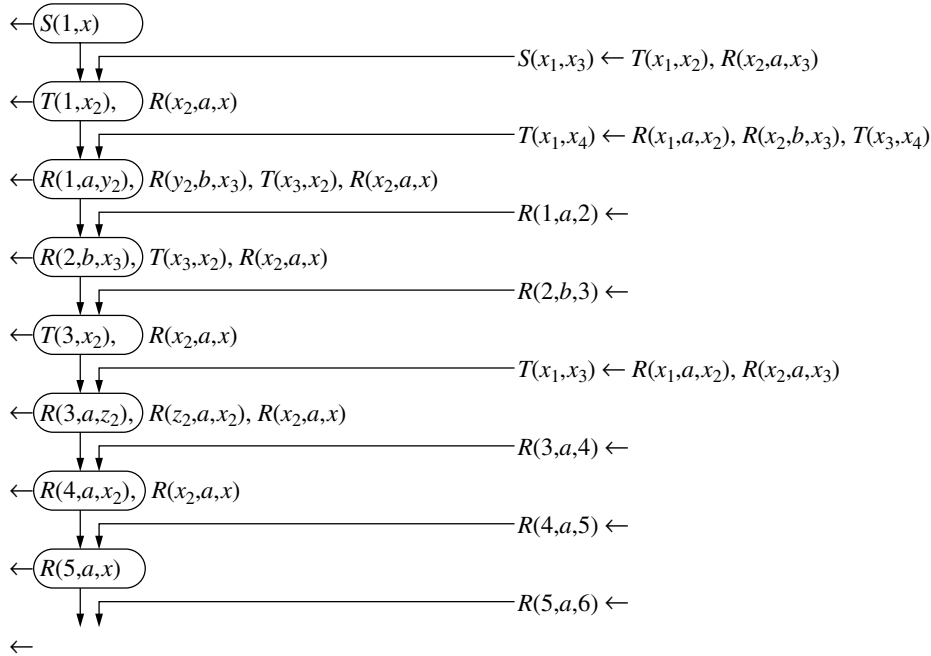
Figure 12.5: SLD refutation
