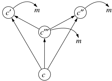
Figure 21.2: Unambiguous definition
