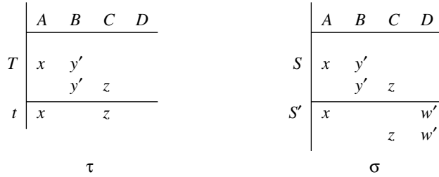
Figure 10.4: Dependencies of Example 10.4.1
