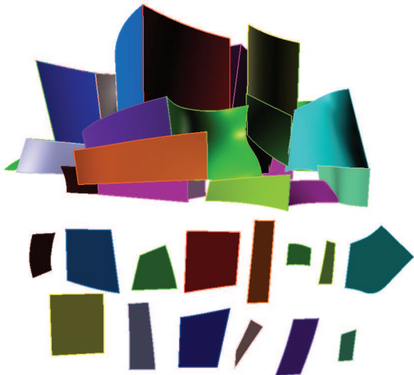
Unrolled surfaces of the front envelope
