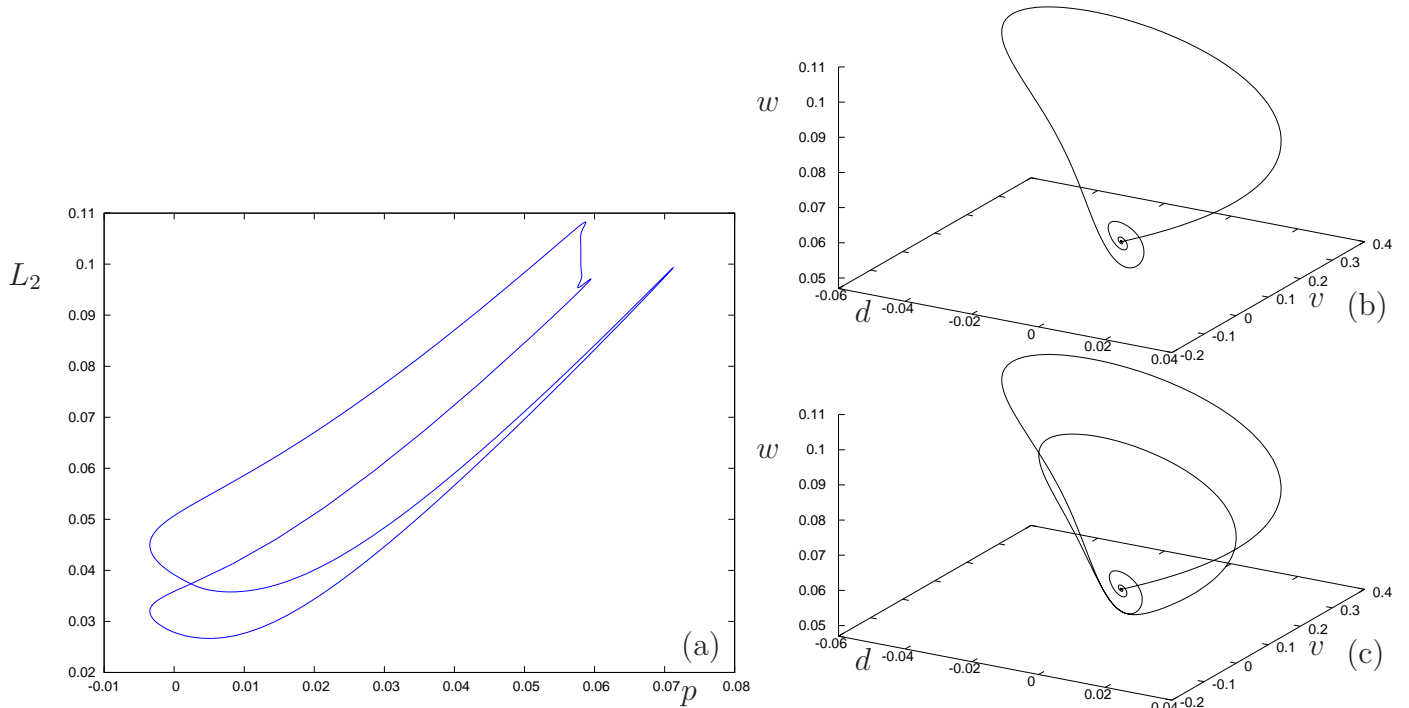
Figure 4: Another projection of the ‘homoclinic banana’ for the FitzHugh-Nagumo system (2) with the parameters (3) (cf. the C curve in Fig. 1). Panels (b) and (c) show two different homoclinic orbits at p \approx 0.06 , s \approx 0.894386 near the lower end of the banana. Note the gross difference in phase space between these two orbits. We (loosely) refer to the orbit in (b) as a single-pulse orbit and the orbit in (c) as a double-pulse orbit.
