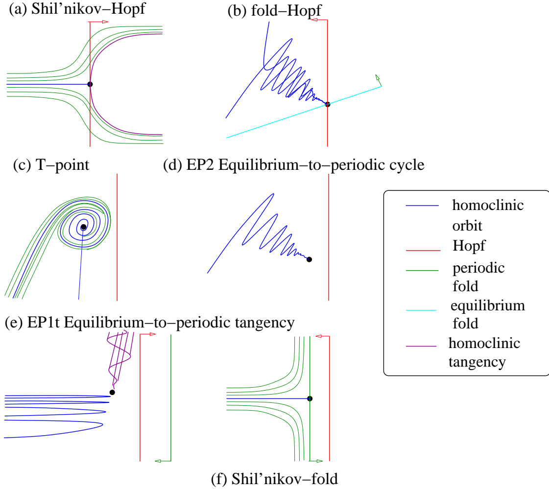
Figure 3: Qualitative unfolding diagrams of six different codimension-two mechanisms that could cause the termination of the homoclinic branch (blue curve) in a CU-system, as it approaches the (red) Hopf curve. The arrows in the figure denote the direction in which the periodic orbit bifurcates from the Hopf bifurcation or from other key bifurcation curves. Note that in full unfoldings of each case there are many more bifurcation curves than those depicted. See text for more details.
