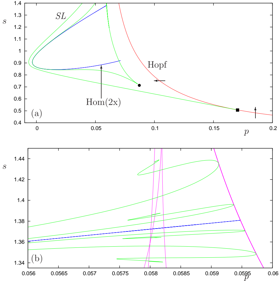
Figure 6: A more detailed bifurcation set for the FitzHugh-Nagumo system. (a) The curve labelled Hom(2x) is the ‘homoclinic banana’ described in the text. The right-most curve is part of the U-shaped Hopf curve, with the square marking a degenerate Hopf bifurcation and the large dot marking a cusp bifurcation. All other curves denote saddle-node bifurcations of limit cycles. The arrows indicate the direction in which periodic orbits appear on the various sections of the Hopf bifurcation curve. (b) A zoom near the top end of the homoclinic curve. The red curve delineates the homoclinic banana. The green curves show saddle-node bifurcations of limit cycles associated with the unfolding of the codimension-one Shil’nikov bifurcation. The purple curves also show saddle-node bifurcations of periodic orbits, but these are associated with the folds on branches of periodic orbits that approach a homoclinic tangency of a periodic orbit (two such saddle-node bifurcations were marked with large dots in Fig. 5).
