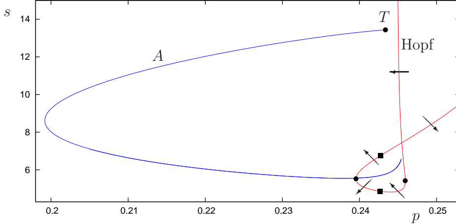
Figure 8: Partial bifurcation set for the SLY-3 model, equations (5), showing the CU nature of the bifurcation curves. The two arms of the Hopf U cross one another, forming a loop, with the arrows denoting the directions in which periodic orbits appear in the Hopf bifurcation. The dots on the Hopf locus denote saddle-node Hopf bifurcations and the squares mark degenerate Hopf bifurcations. The C-shaped homoclinic bifurcation curve (labelled A following the notation of [41]) terminates at the top at a T-point (labelled T), and turns around sharply at the lower end in the same way as the lower end of the C curve in the FitzHugh-Nagumo equations.
