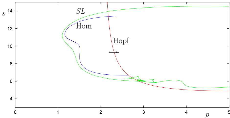
Figure 11: Partial bifurcation set for the nine-dimensional calcium model, equations (7). The C curve of homoclinic bifurcations appears to cross the Hopf bifurcation curve at one end, but this is believed to be a numerical artifact as explained in the text. At the other end, the C curve turns around sharply at the first in a sequence of sharp turns which are not visible in this figure. There are no degenerate points on the Hopf locus; the saddle-node bifurcation of limit cycles (curve marked SL) does not terminate in this figure.
