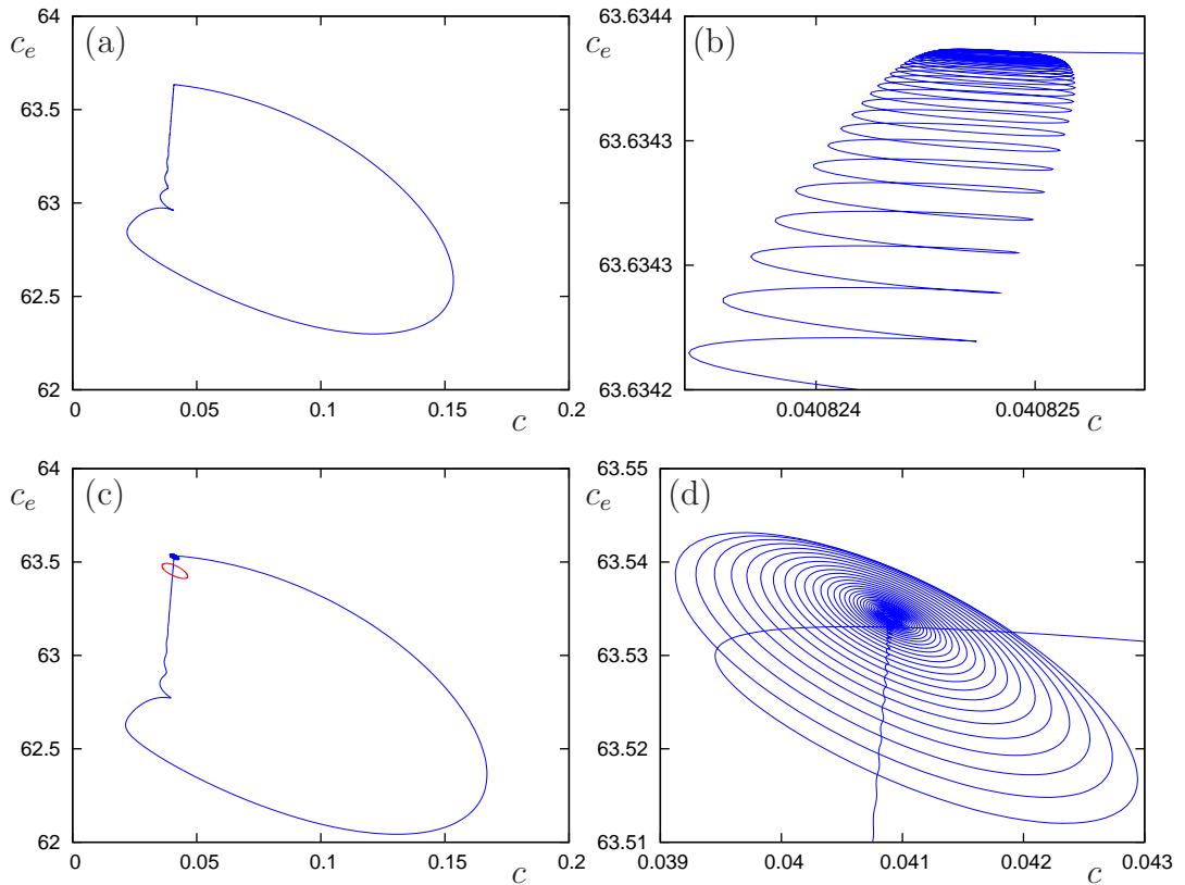
Figure 16: Phase portraits at the points labelled (i) and (ii) in Fig. 15, computed with AUTO by following an orbit of fixed period (period 5000) with AUTO constant NTST=1000 . (a) At point (i); (b) enlargement of (a) near the equilibrium. (c) At point (ii). The red curve is the periodic orbit created in the Hopf bifurcation; (d) enlargement of (c) near the equilibrium.
