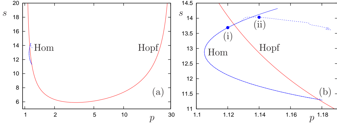
Figure 15: (a) Partial bifurcation set for the five-dimensional model, equations (9). (b) An enlargement of part of (a). Homoclinic and Hopf bifurcations are labelled. The points labelled (i) and (ii) in (b) correspond to the parameters used for the phase portraits in Fig. 16. In (b) two different algorithms are used to compute the homoclinic curve: projection boundary conditions (solid line) and fixed period-5000 periodic orbit (dashed line). To the left of the Hopf line these two curves are overlaid to the accuracy depicted.
