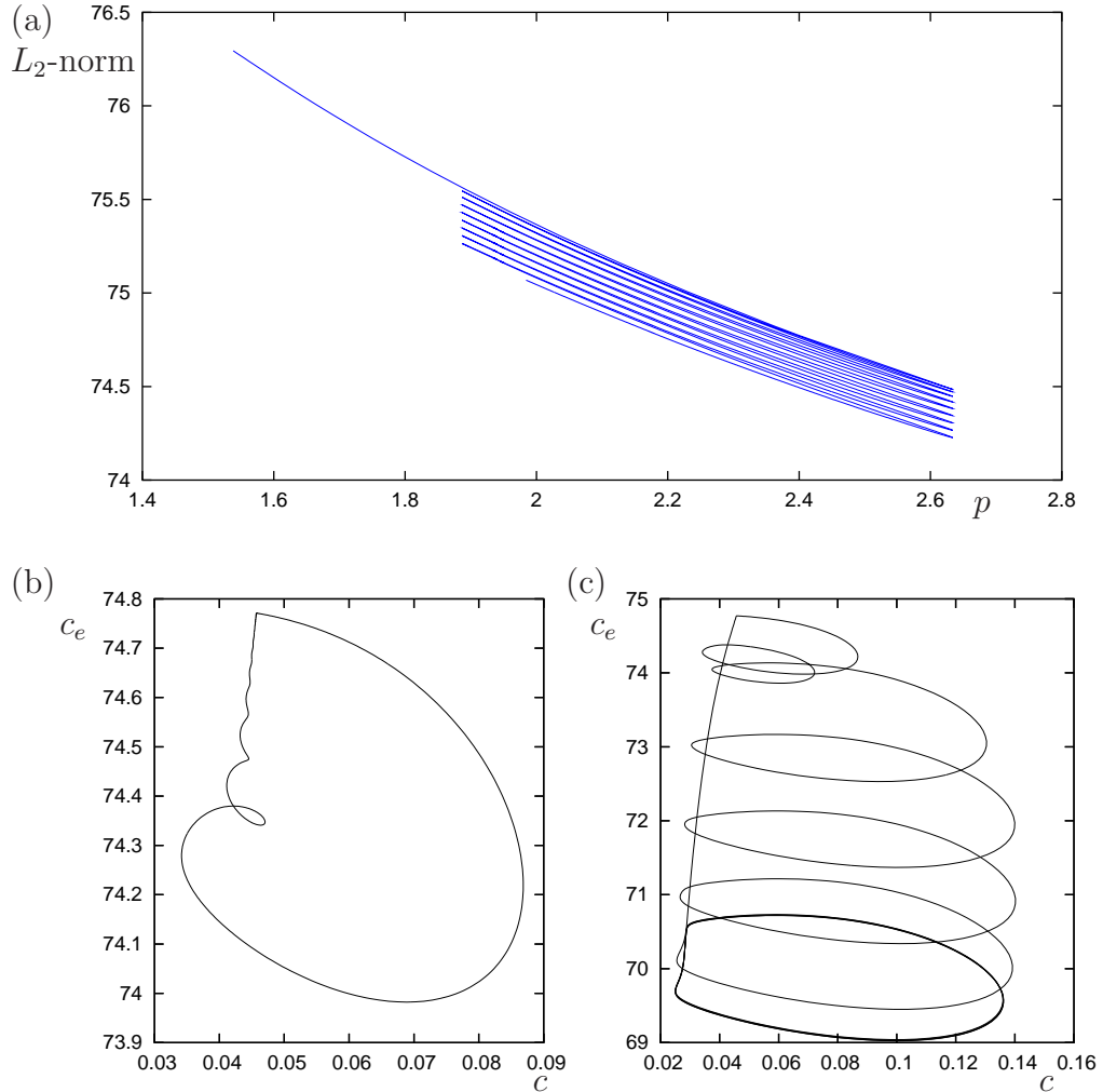
Figure 12: (a) Detail along the lower part of the homoclinic branch in Fig. 11, showing the L_2 -norm of the homoclinic orbit as a function of p . The turning points on the homoclinic branch initially approximately alternate between two locations, with p values given approximately by 2.63466, 1.88681, 2.63383, 1.88681, 2.63383 and 1.88681, and then follow a repeated sequence of six values of p : 2.63383, 1.93415, 1.93954, 1.88681, 1.95014, 1.94495. Not all turning points can be distinguished in the figure. Below: Homoclinic orbits near the lower end of the homoclinic branch. (b) The homoclinic orbit before going through any turning points, at (p, s) = (2.4, 6.68342) ; (c) the homoclinic orbit at approximately the same place in parameter space, at (p, s) = (2.4, 6.68342) after going through 17 outer turning points.
