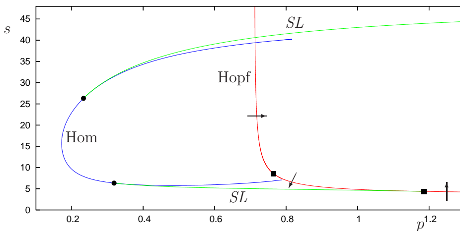
Figure 13: Partial bifurcation set for the four-dimensional calcium model, equations (8). The homoclinic bifurcation curve appears to cross the Hopf locus at the top end, but this is believed to be a numerical artifact, as discussed in the text. At the lower end the homoclinic locus goes through a sequence of sharp turning points, eventually converging at a codimension-two point at p = 0.7682935 . The two curves of saddle-node bifurcations of periodic orbits (marked SL) terminate on the homoclinic bifurcation curve at the large dots where the leading eigenvalues of the corresponding equilibrium resonate: the saddle quantity of the saddle vanishes at these points. The lower SL bifurcation terminates at its right end at a degenerate Hopf bifurcation, indicated by a square. A second degenerate Hopf bifurcation lies to the left, just above the lower end of the C curve; the SL curve emanating from this degenerate Hopf bifurcation is not shown. The arrows indicate the direction of the Hopf bifurcation as in Fig. 6.
