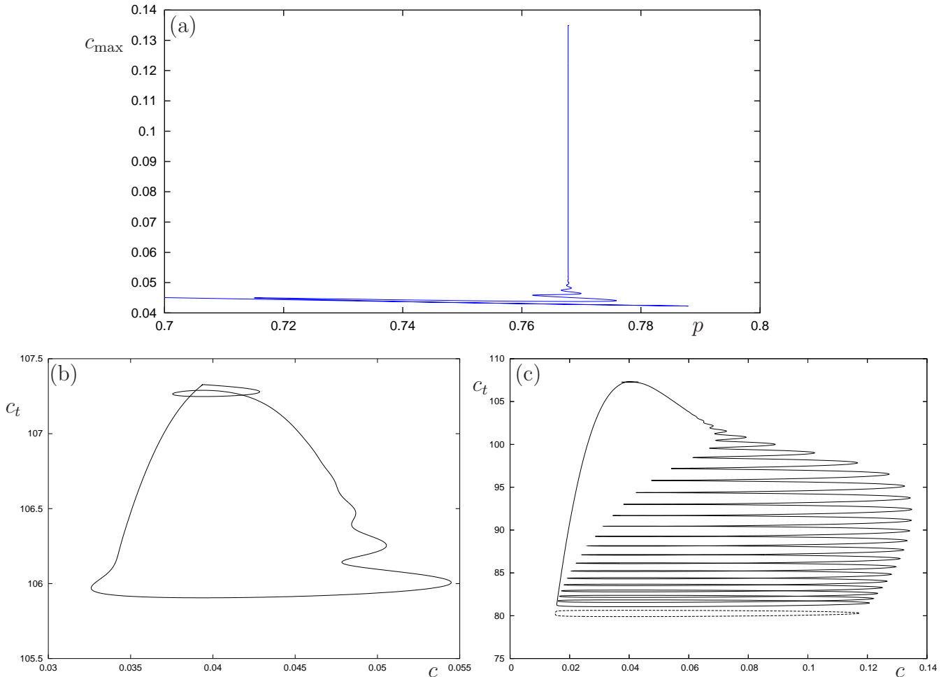
Figure 14: (a) The lower part of the homoclinic bifurcation curve in the four-dimensional calcium model, equations (8), showing the maximum value of c on the homoclinic orbit, c_{\max} , as a function of p . After many turns c_{\max} stabilises at 0.134922. (b) The homoclinic orbit at p = 0.7682935 after 15 turns of the homoclinic bifurcation curve. (c) The homoclinic orbit at p = 0.7682935 after many turns of the homoclinic bifurcation curve. Also plotted (dashed curve) is a periodic orbit that bifurcates from the right arm of the U-shaped Hopf locus. This orbit was obtained by continuing in p for s fixed from the Hopf bifurcation point at (p, s) = (22.04131, 6.878683) .
