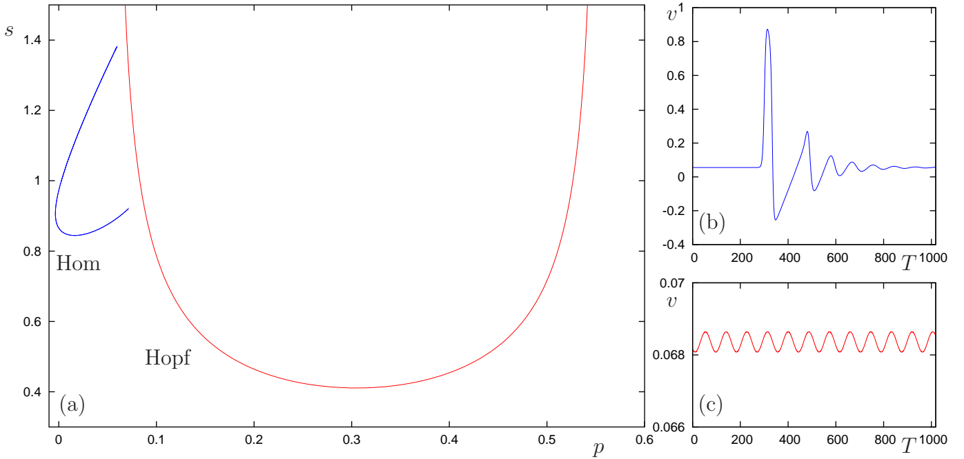
Figure 1: (a) Partial bifurcation set for the travelling wave FitzHugh-Nagumo equations (2) for the parameter values given in (3), illustrating the U-shaped curve of Hopf bifurcations and C-shaped curve on which homoclinic orbits occur. Panel (b) shows a time series for a homoclinic orbit near the top of the C branch, at (p, s) = (0.0575862, 1.37) . Panel (c) shows a time series for a nearby periodic orbit, at (p, s) = (0.0703753, 1.37) ; this periodic orbit is created in a Hopf bifurcation on the U branch.
