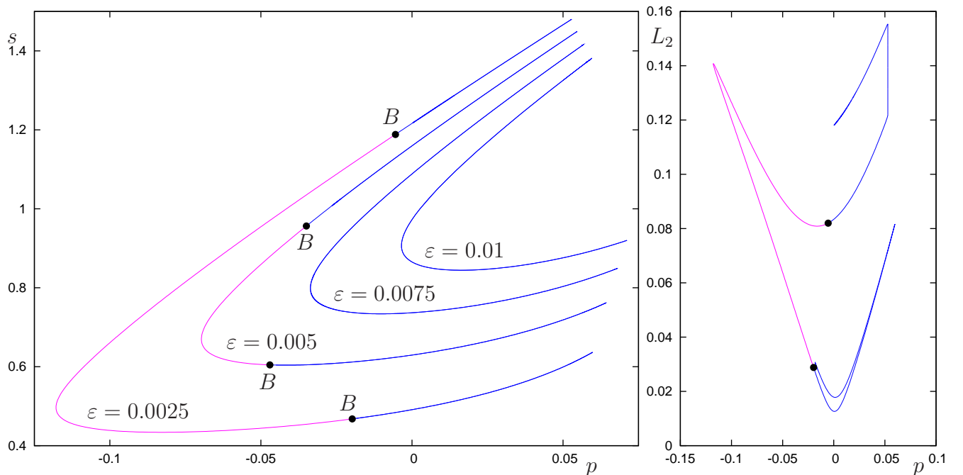
Figure 7: Homoclinic bifurcation curves in parameter space for different values of \varepsilon in the FitzHugh-Nagumo system. There exist Belyakov transitions (marked B ) on the curves corresponding to \varepsilon = 0.0025 and \varepsilon = 0.005 (the banana-split case), whereas on the other curves no Belyakov transitions occur (the banana case). On the left side of the Belyakov points the eigenvalues of the equilibrium are real rather than complex. Right: L_2 -norm for the homoclinic orbits occurring along the banana-split curve in the case \varepsilon = 0.0025 . This panel demonstrates that each point on the C-shaped curve between the Belyakov points corresponds to a single homoclinic bifurcation curve, while to the right of each Belyakov point there are two curves of homoclinic bifurcations.
