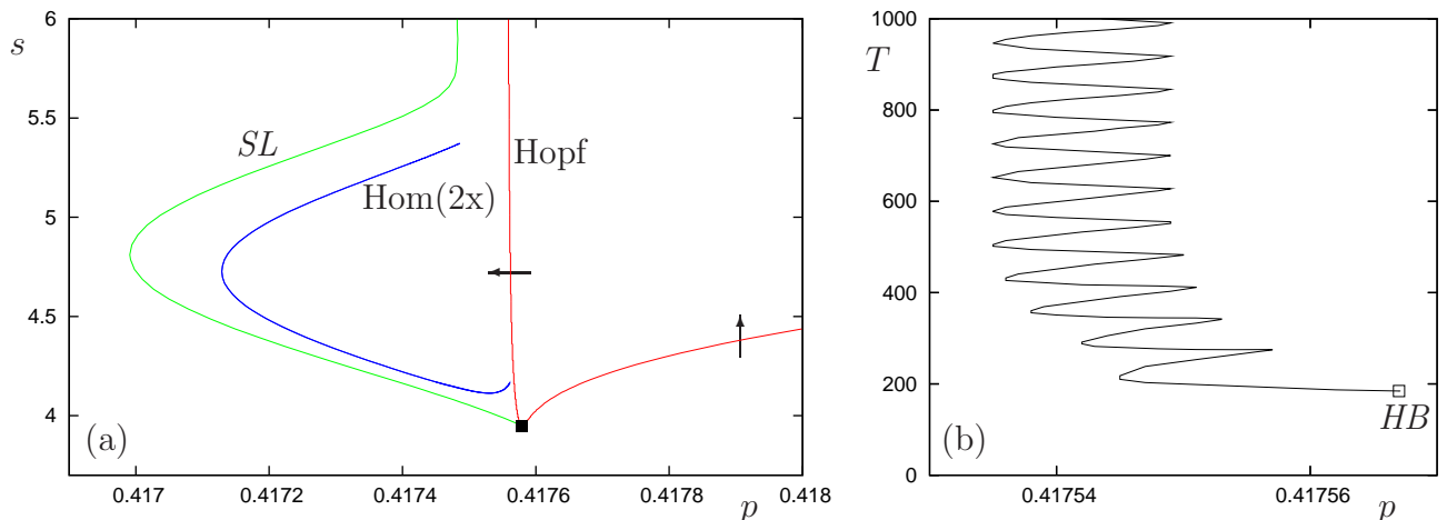
Figure 10: (a) A partial bifurcation set for the SLY-4 model, equations (6). The curve labelled Hom (2x) represents a homoclinic banana. The square on the Hopf curve marks a degenerate Hopf bifurcation. All other curves are saddle-node bifurcations of limit cycles. The arrows through the Hopf locus indicate the direction in which periodic orbits appear on the various sections of the Hopf bifurcation curve. (b) Bifurcation diagram for the SLY-4 model, for s = 4.17 , showing the branch of periodic orbits that emanates from the Hopf bifurcation in panel (a).
