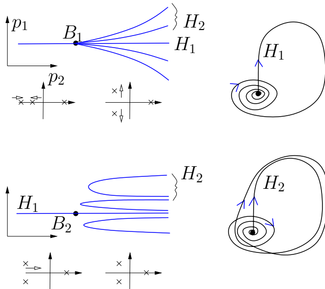
Figure 2: Partial unfoldings of two Belyakov transitions in the (p_1, p_2) parameter plane. Here p_1 unfolds the existence of a primary homoclinic orbit H_1 whereas variation of p_2 causes the homoclinic bifurcation to change from the tame case to the Shil'nikov case. In the upper panel, the Belyakov point B_1 is caused by a pair of non-semisimple eigenvalues coalescing on the real axis and becoming complex. In the lower panel the saddle quantity \sigma changes sign. In both cases, infinitely many N -pulse homoclinic orbits are created in the neighbourhood of the B -points, represented here by a few curves of double-pulses H_2 . There are also infinitely many curves of period-doublings and folds of periodic orbits that are not depicted.
