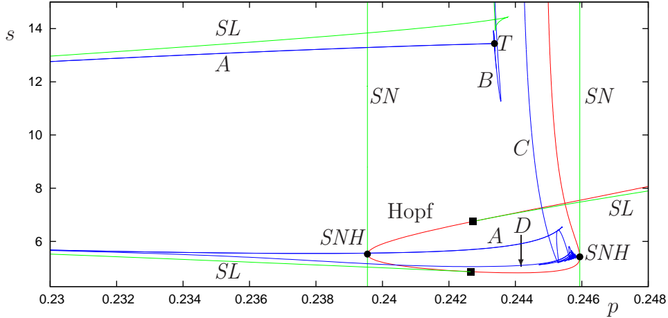
Figure 9: A more detailed bifurcation set for the SLY-3 model. This figure is an enlargement of part of Fig. 8. Depicted are the homoclinic bifurcations A, B, C, and D, the two saddle-node bifurcations of equilibria SN, the two saddle-node Hopf bifurcations SNH, the T point, and the two saddle-node bifurcations of limit cycles SL which terminate at the degenerate Hopf bifurcations marked with squares.
